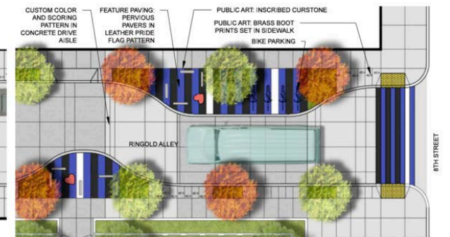
3 8TH STREET & RINGOLD DETAIL PLAN SCALE: 1" = 10'-0"
