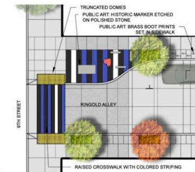
2 9TH STREET & RINGOLD DETAIL PLAN SCALE: 1" = 10'-0"
