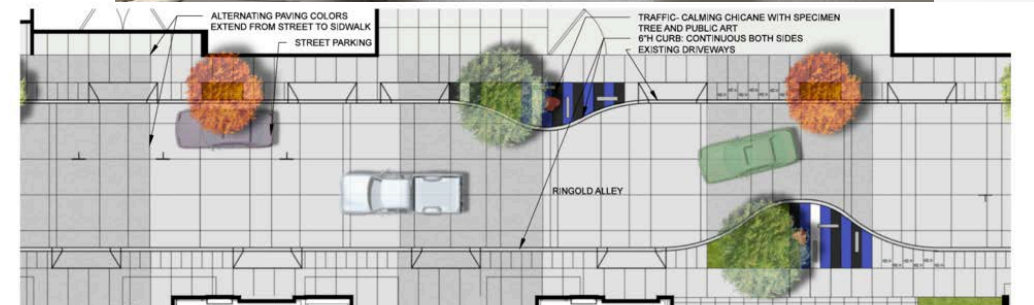
1 MID-BLOCK RINGOLD DETAIL PLAN SCALE: 1" = 10'-0"
